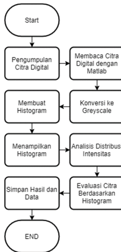
Gambar 3. Flowchart Histogram
